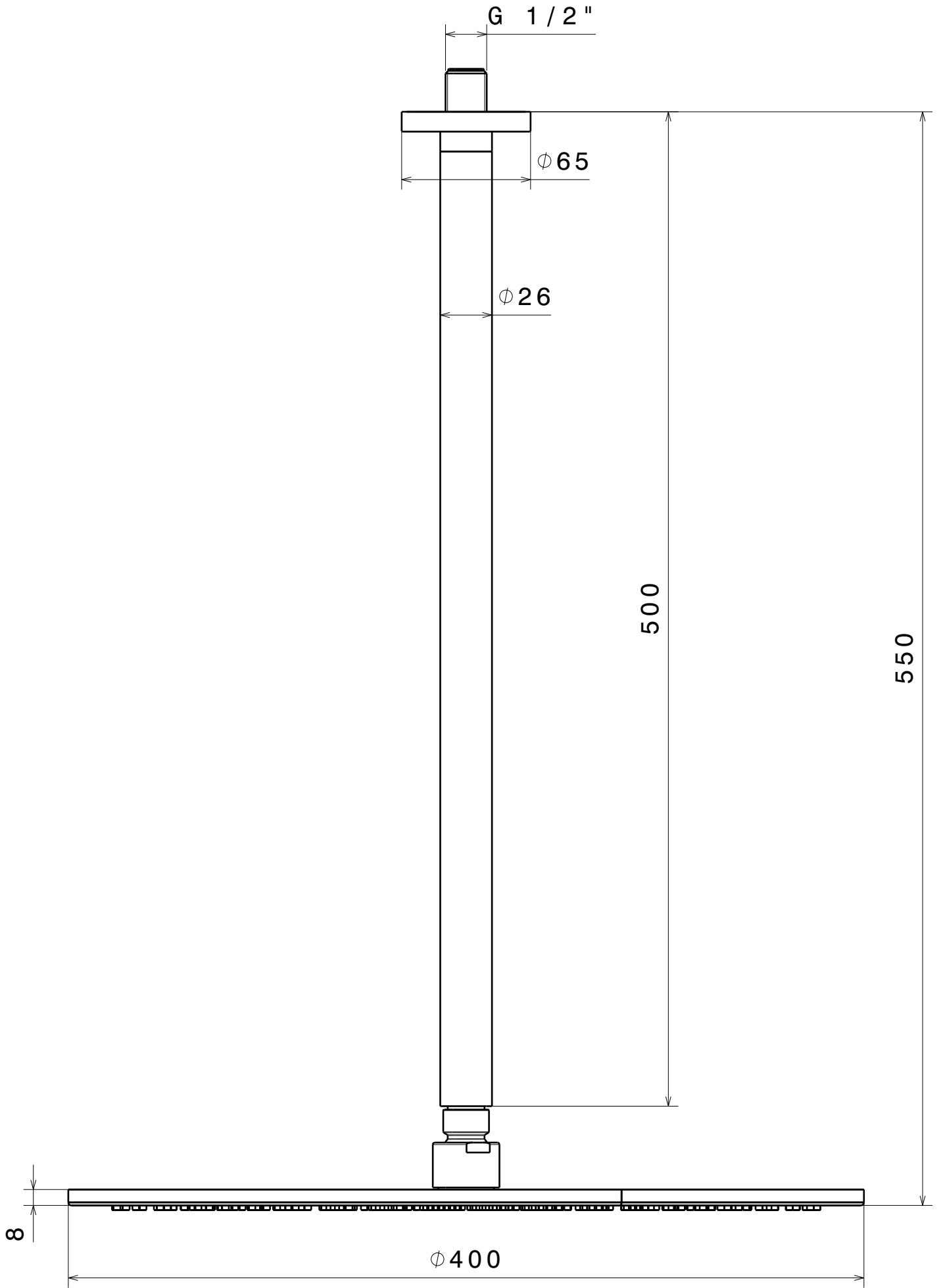
HEAD SHOWER '67753'
