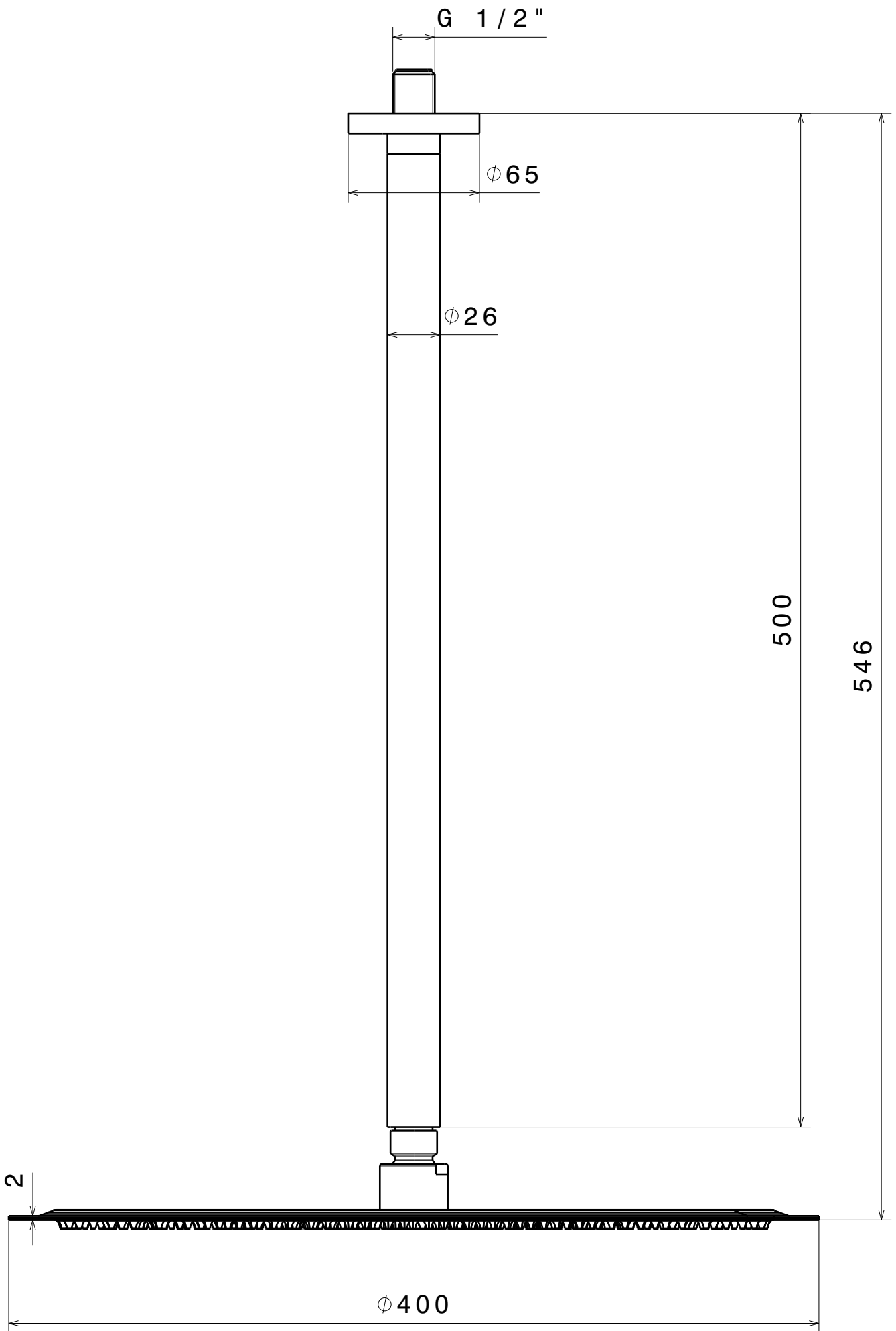
HEAD SHOWER '67771'
