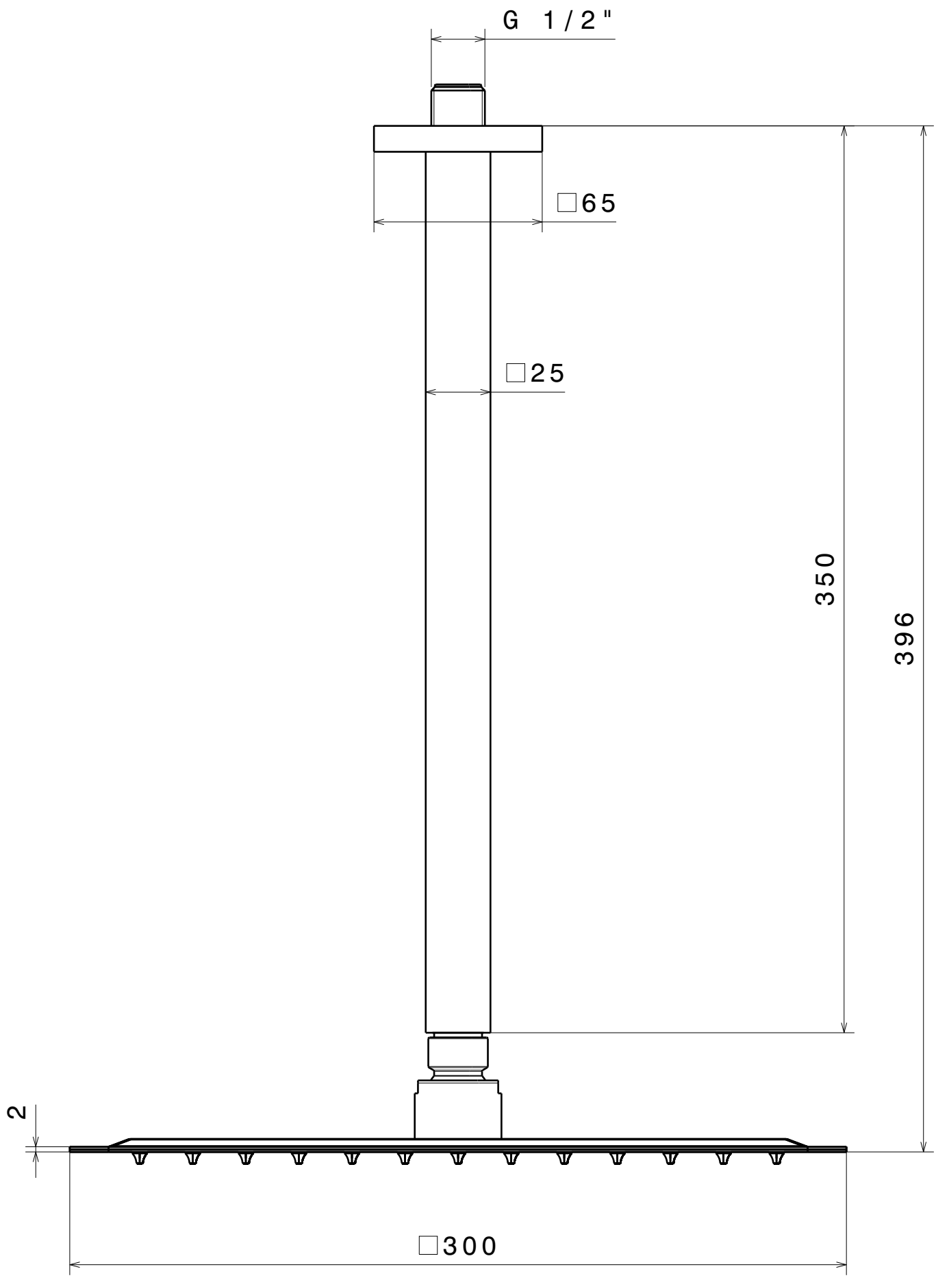
HEAD SHOWER '67776'
