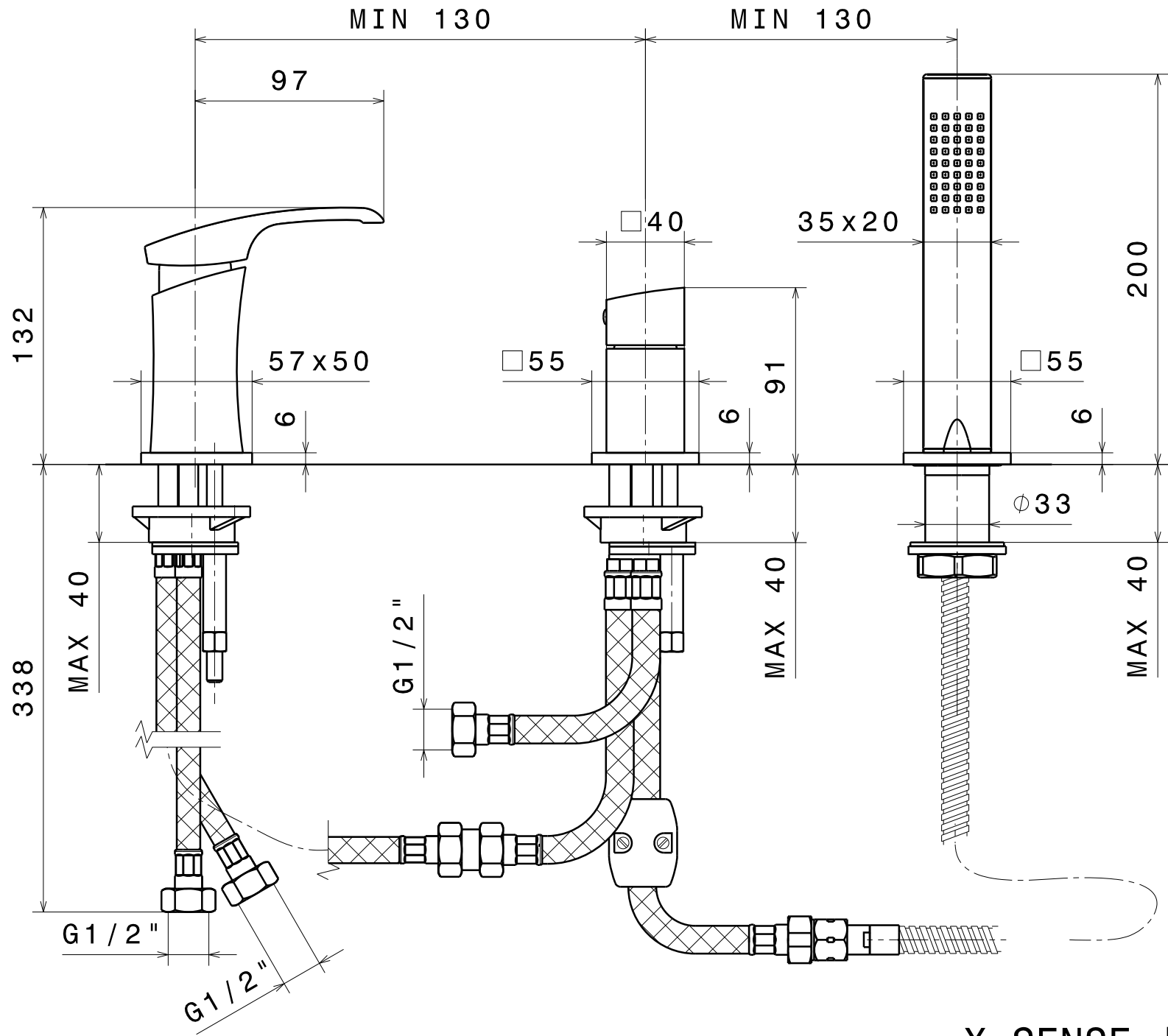
X-SENSE '62581C'
